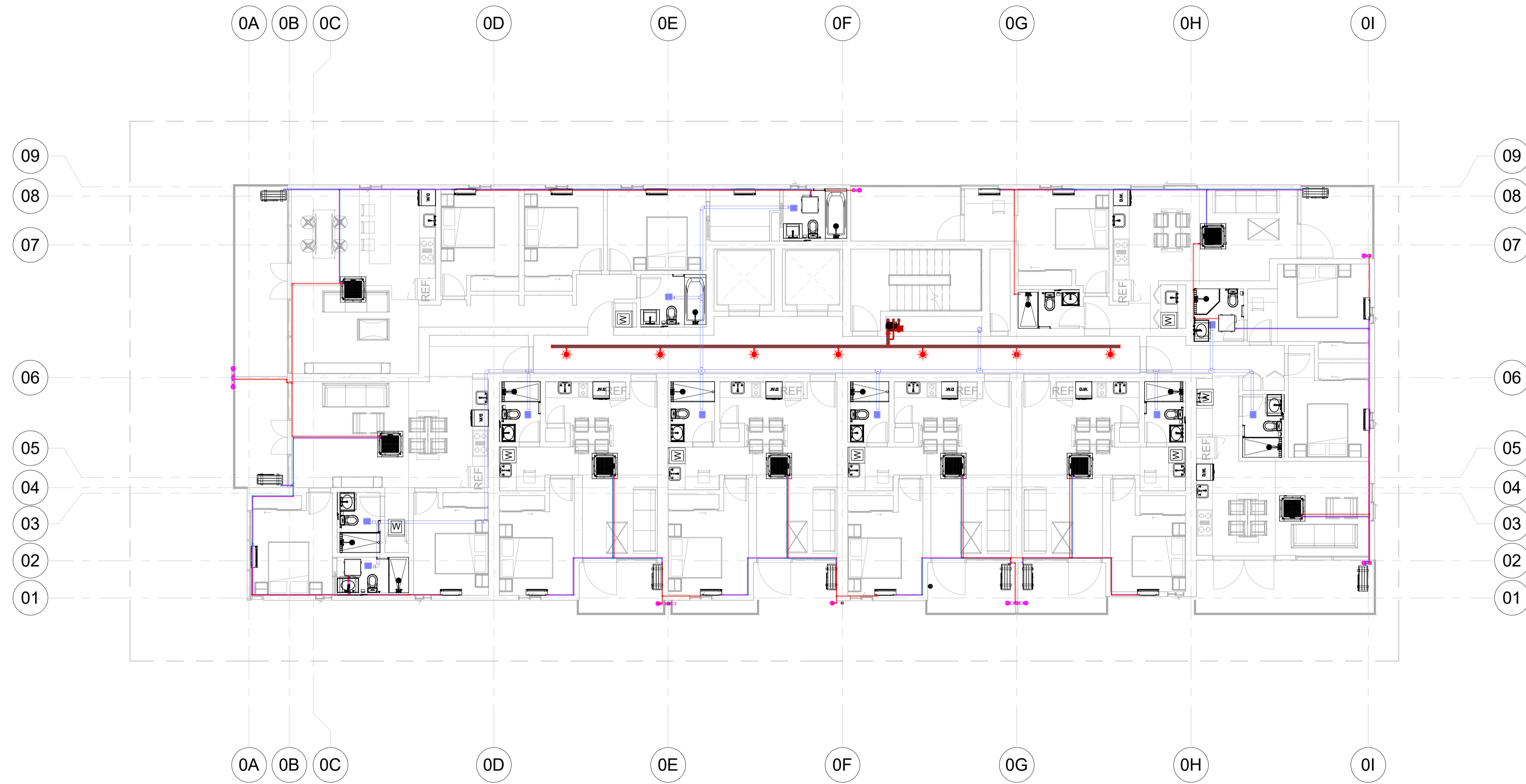
1 04-EM-First Floor 1 : 100
